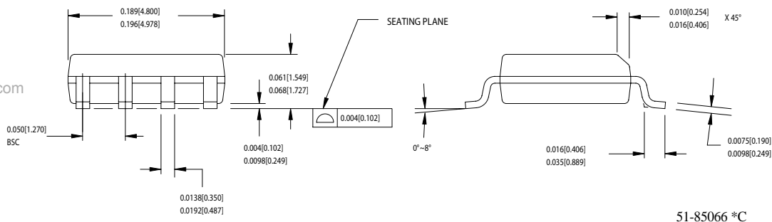
Figure 4-1. 8-Lead (150-Mil) SOIC
